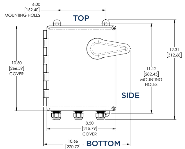
Dimensions of MVP Main Disconnect enclosure.
