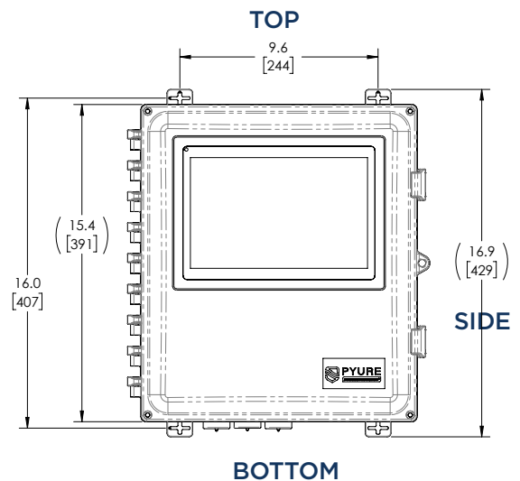
Dimensions of Pyure Insight Edge 1101 Gateway, with HMI.
