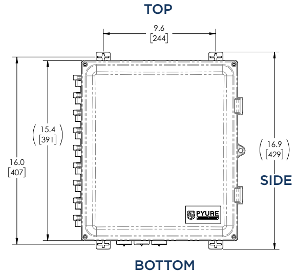
Dimensions of Pyure Insight Edge 1100 Gateway.
