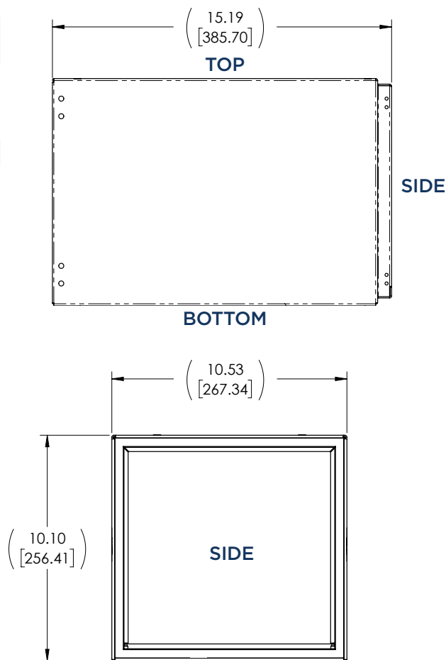
Dimensions of IDI In-Line Dynamic Enclosure.
