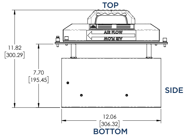
Dimensions of IDI03 unit.
